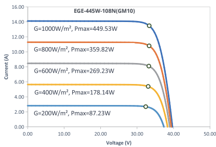
IV-Curves Irradiance
