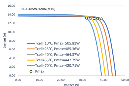
IV-Curves Temperature
