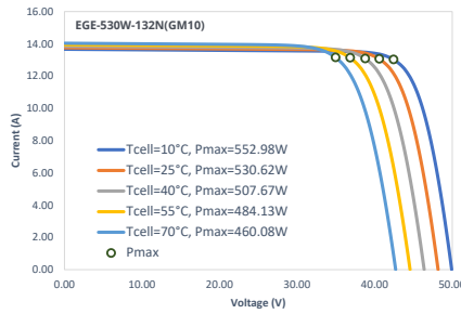
IV-Curves Temperature
