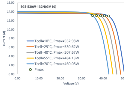
IV-Curves Temperature
