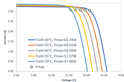
IV-Curves Temperature
