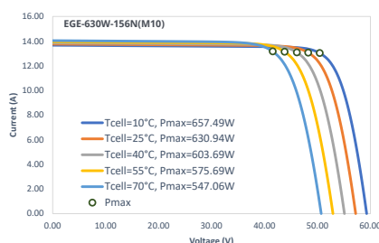
IV-Curves Temperature
