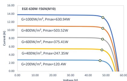
IV-Curves Irradiance
