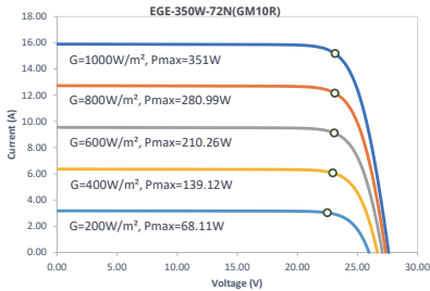
IV-Curves Irradiance
