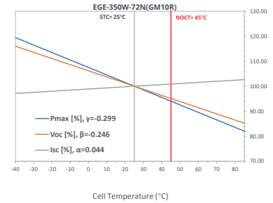
Temperature Dependence of Isc, Voc, Pmax
