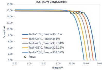
IV-Curves Temperature
